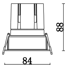
Φ75mm RECESSED
