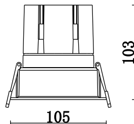
Φ95mm RECESSED
